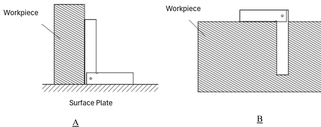
Figure 2 Instructions for Using the Engineer's Square
